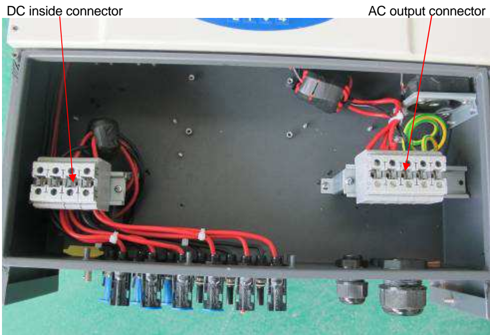
Internal view of the unit
